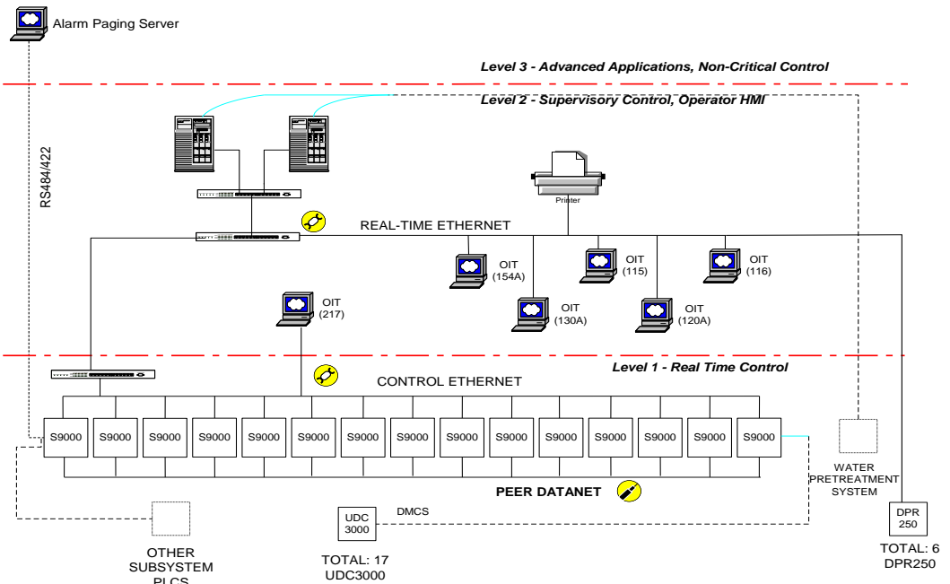
Topology of the Building 211 Honeywell System Upgrade
